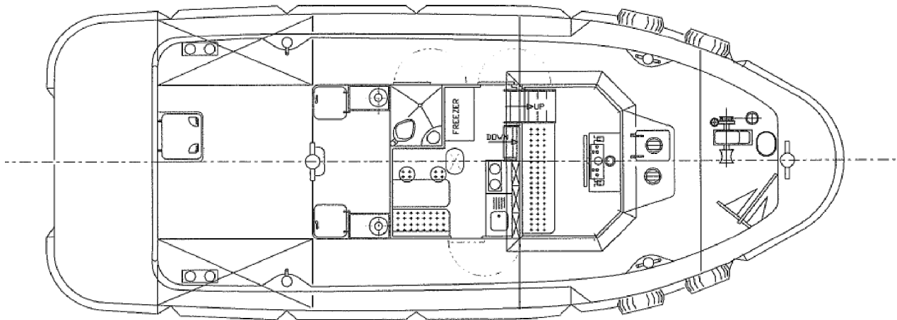
DECK PLAN
