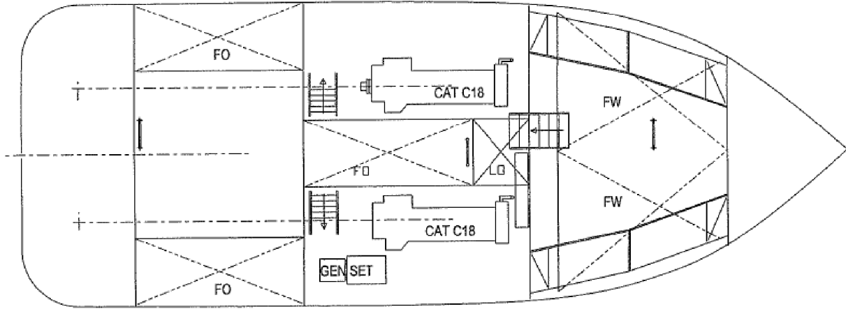
LOWER DECK PLAN
