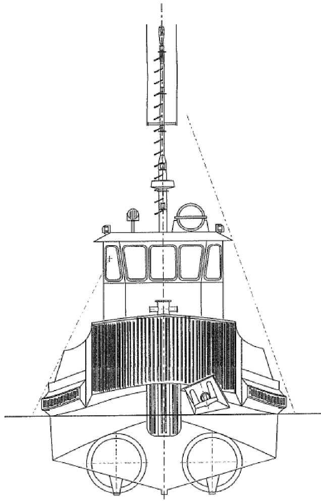
BOW VIEW
